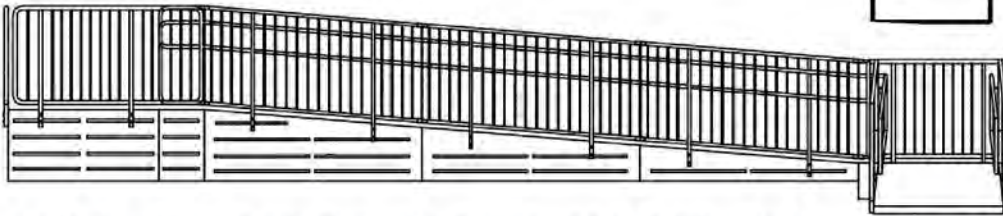
5 HI L-TURN RAMP W/ INTERMEDIATE LANDING TO ACCESS UP TO 35" IN HEIGHT.
