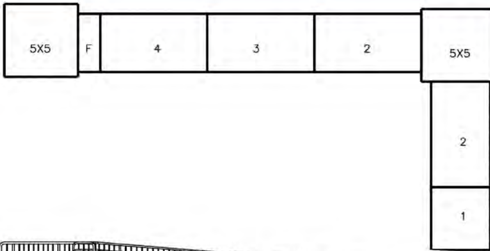
5 HI RAMP W/ INTERMEDIATE LANDING TO ACCESS UP TO 35" IN HEIGHT.
