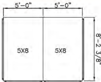
5' X 8' 2 3/8" DECKING SECTIONS FOR ELEVATED WALKWAYS OR SIDEWALKS .
