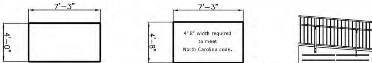
TO ACCESS UP TO AN ADDITIONAL 7.25" IN HEIGHT PER SECTION.
