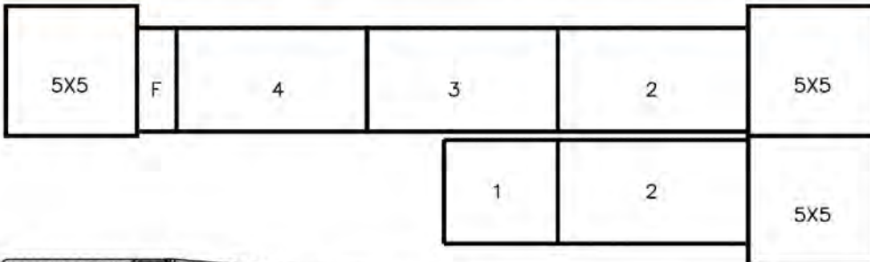
5 HI L-TURN RAMP W/ INTERMEDIATE LANDING TO ACCESS UP TO 35" IN HEIGHT.
